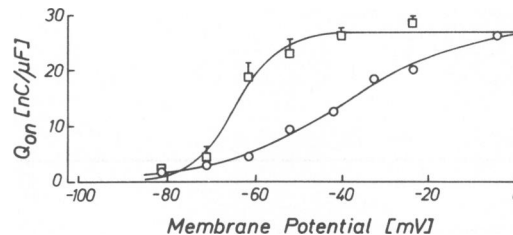
FIGURE 3 Effect of 8 mM \text{ClO}_4^- on charge movement during depolarizing pulses of 100 ms duration. Circles (○) and squares (□) give the mean values of Q_{\text{ON}} obtained from 5 fibers in the absence and presence of \text{ClO}_4^- , respectively. Error bars give SEM. The curves were drawn according to Eq. 1, with the parameter values given in Table I. The temperature was 2\text{--}4^\circ\text{C} .
